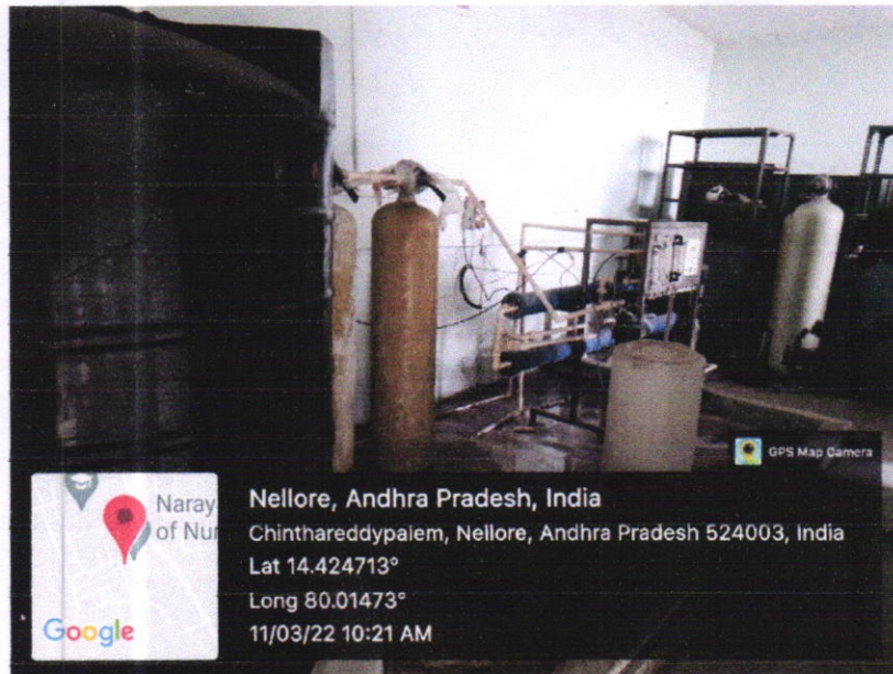
Fig: RO plant for Water Purification
